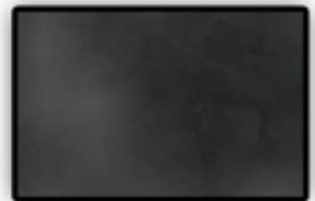
Black Hole CR-424
