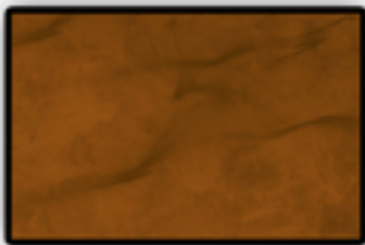
Pillars of Creation CR-497
